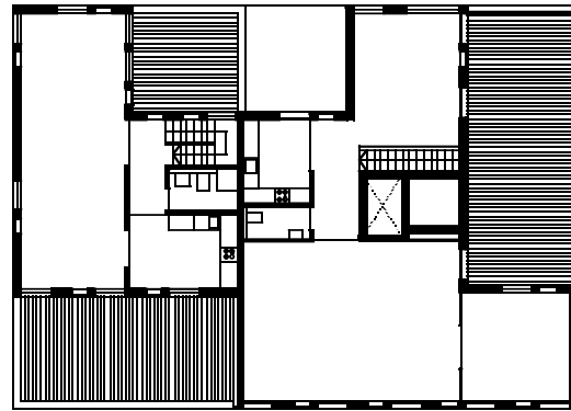
Planta séptima Seventh floor plan
