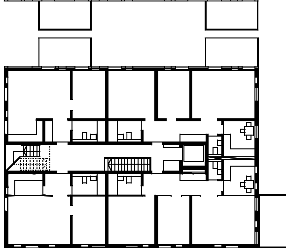
Planta segunda Second floor plan
