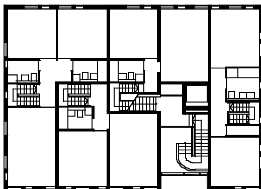
Planta baja Ground floor plan
