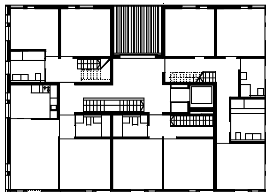
Planta sexta Sixth floor plan
